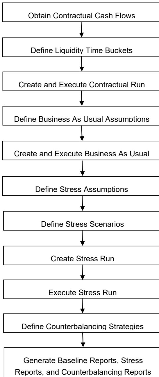
Figure 1 LRS Process Flow
